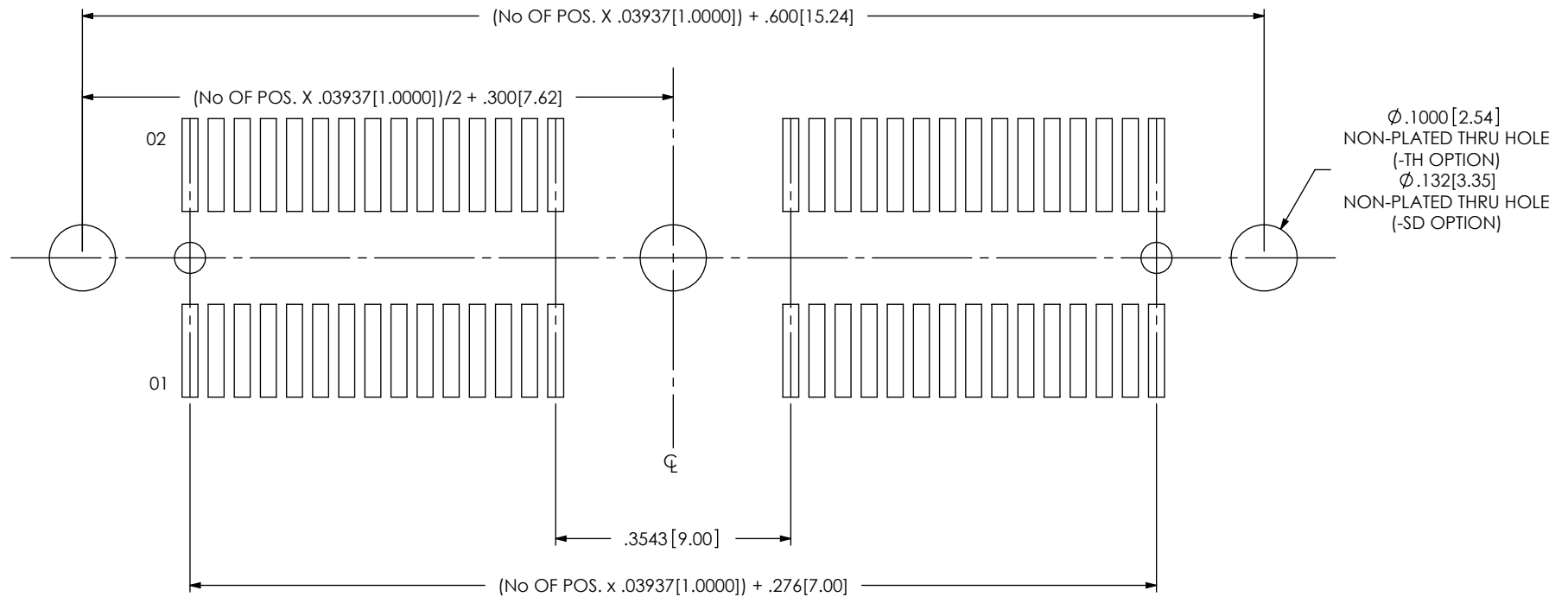
FIG. 2 FOR -40 AND -50 POS (THREADED) ALL OTHER DIMENSION ARE THE SAME AS ABOVE
